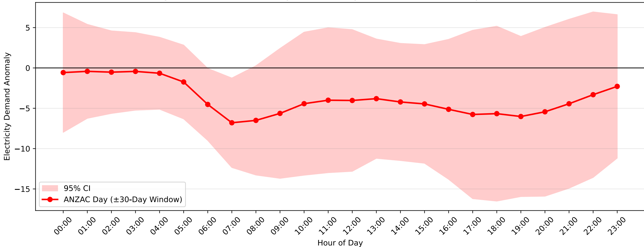
Kogarah Demand Anomaly: ANZAC Day (2010-2011, \pm 30 -Day Window)
