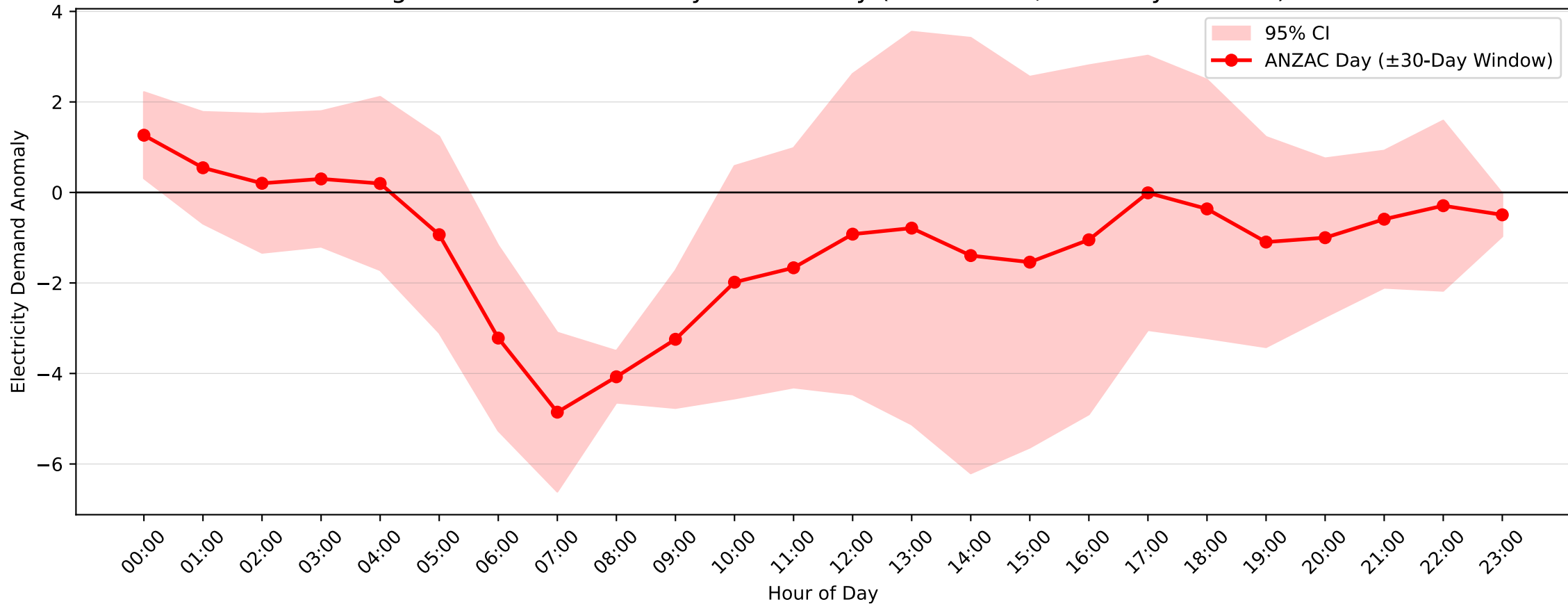
Kogarah Demand Anomaly: ANZAC Day (2016–2017, \pm 30 -Day Window)
