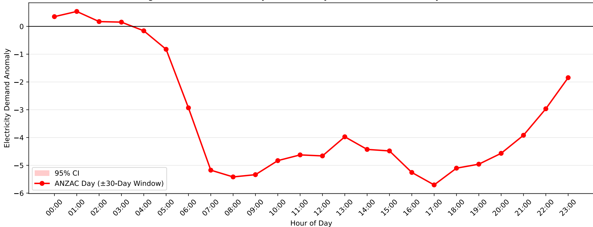
Kogarah Demand Anomaly: ANZAC Day (2009–2010, \pm 30 -Day Window)
